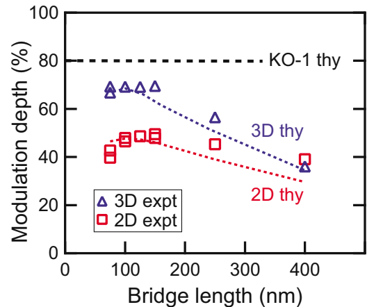
FIG. 4. (Color online) Critical current modulation depth as a function of device length for both 3D and 2D nanobridges. The thick dashed line at the top is the theoretical prediction for an ideal weak link SQUID at zero temperature with zero loop inductance. The thinner dashed lines are numerical calculations for our 3D (middle line) and 2D (lower line) devices, including the effect of finite loop inductance.
