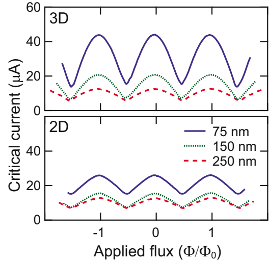
FIG. 3. (Color online) Critical current as a function of applied magnetic flux for 75, 150, and 250 nm long nanoSQUIDs. The upper panel shows experimental results for nanobridges with 3D banks and the lower panel for 2D banks.
