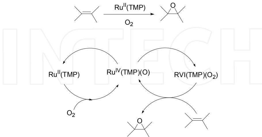
Scheme 9. Ru(TMP)-catalyzed olefins epoxidation with dioxygen
